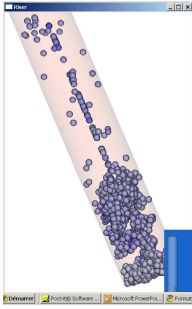
Figure 4: Another view during runtime. The spheres represent the solid macro-particles. We can see an emerging privileged solid path near the axis of the riser cylinder. At the bottom of the cylinder, one can see a strong concentration of solid catalyst particles that form the fluidized bed.
